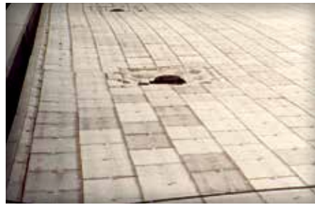
Figure 4. Some ballast-type slabs for roof decks are made with lightweight concrete materials. They can be joined with tongue-and-grooves and/or with connectors to resist wind uplift. This is one of several designs available.
