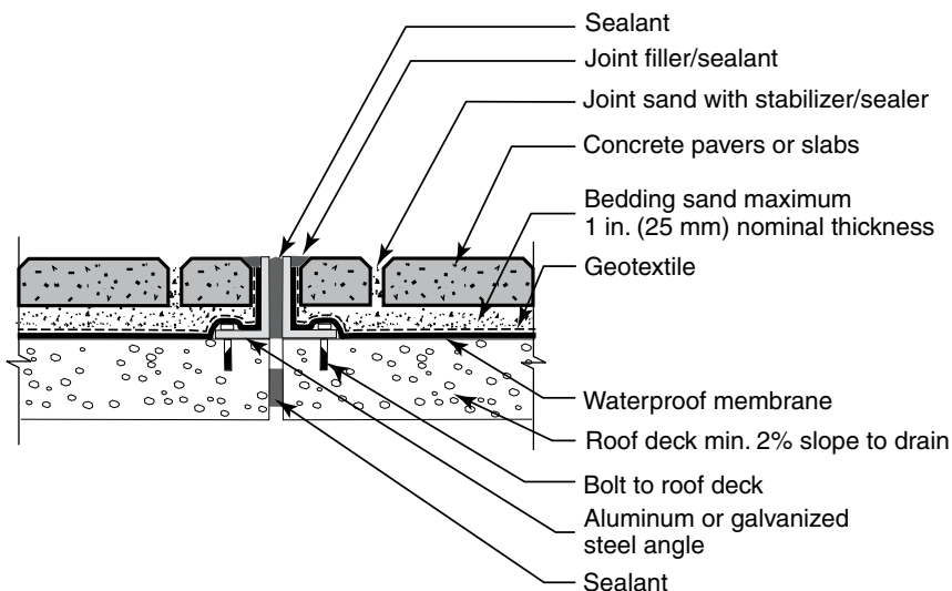
Figure 12. Edge restraint detail at a roof construction joint for pedestrian roof applications (14)
